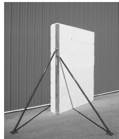
PANELJACK CORNER BRACE
